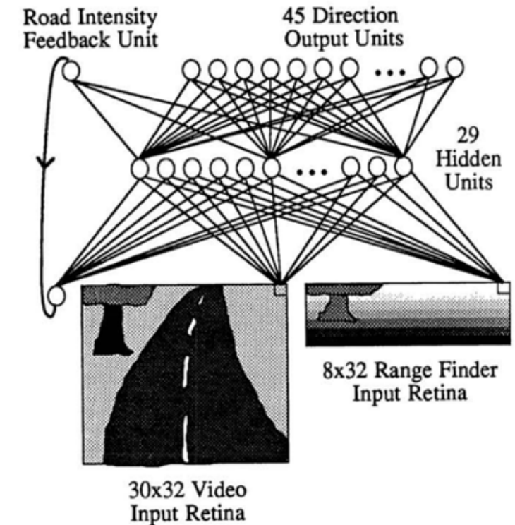
Figure 1: ALVINN Architecture
